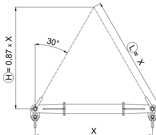
Dimensions at 30°
